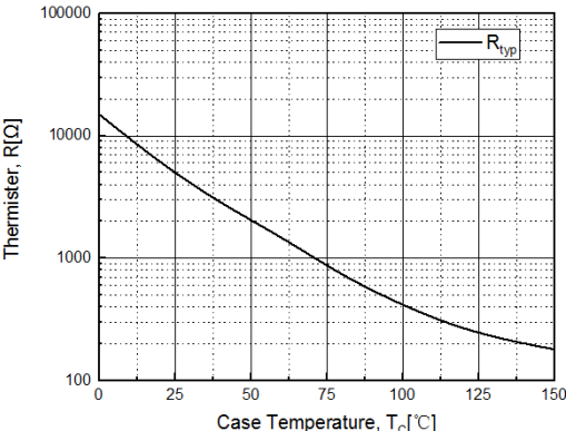
Fig. 10. NTC-Thermistor-temperature characteristic
