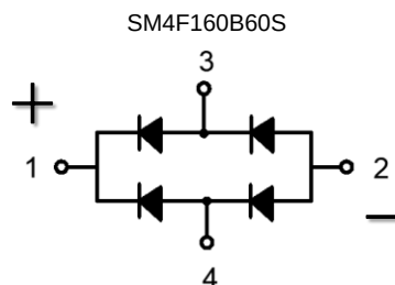
Internal Circuit
