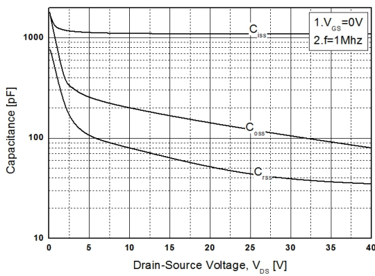
Fig. 5. Capacitance Characteristics
